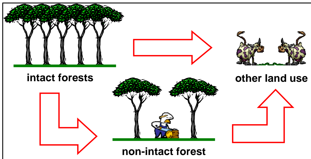
Figure 2.2.4. Forest conversions types considered in the accounting system.
