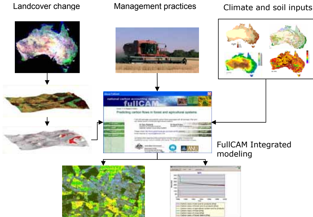
Figure 3.1.3. Graphical depiction of the NCAS modeling framework.
