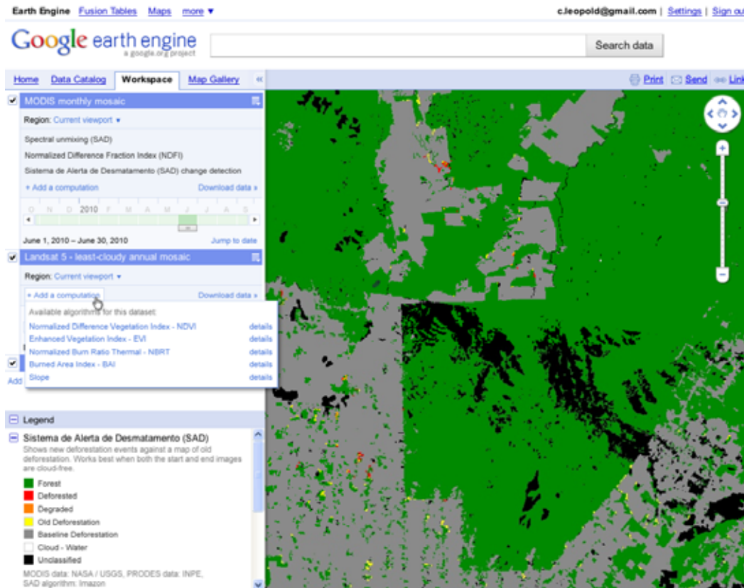
Figure 2.9.3. Results of running Imazon's forest change analysis in Google Earth Engine on satellite imagery taken between March and June, 2010. The green color represents forested areas, while the red and yellow areas indicate recent deforestation. The analysis indicates that no deforestation took place inside the Surui territory during this period, whereas along the perimeter and outside of their territory there is evidence of recent deforestation.
