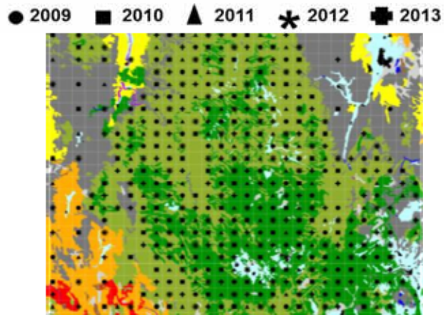
Figure 3.3.5. Each year 20% of permanent plots are resampled systematically.
