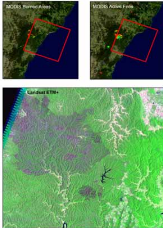
Figure 2.5.4. Large fire in an open Eucalyptus forest in South East Australia, October 2002. The ground fire is only partially detected by the coarse/moderate resolution MODIS products (top row). On the basis of the information given by such products it is possible to select the time and location for higher resolution imagery (Landsat ETM+ data, bottom row) that allows mapping burned area with c. 0.1 ha spatial resolution.
