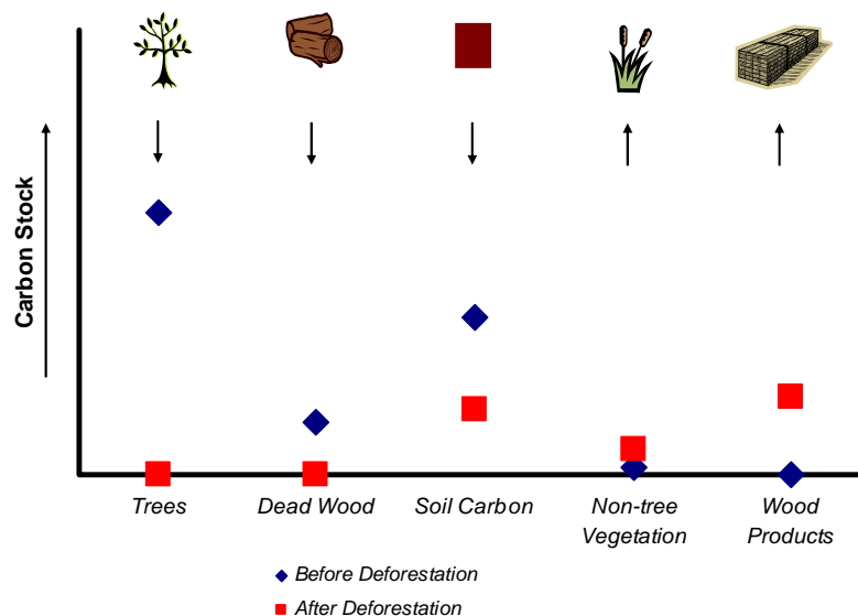
Figure 2.3.1. Fate of existing forest carbon stocks after deforestation.
