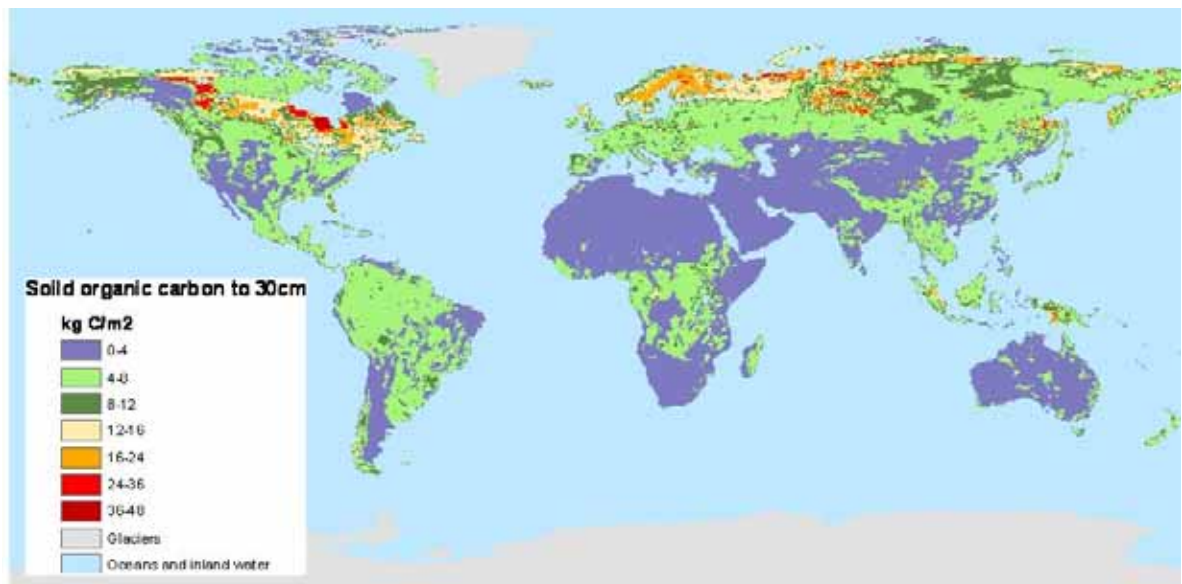
Figure 2.3.4. Soil organic carbon map (kg/m 2 or x10 t/ha; to 30 cm depth and 0.5° resolution) from the global map produced by the USDA Natural Resources Conservation Service.
