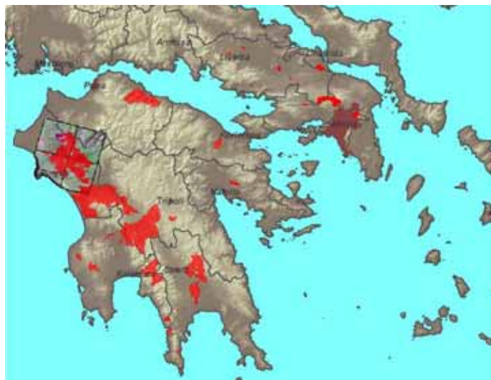
Figure 2.5.6. Overview of the Burned areas over the Peloponnesus.
