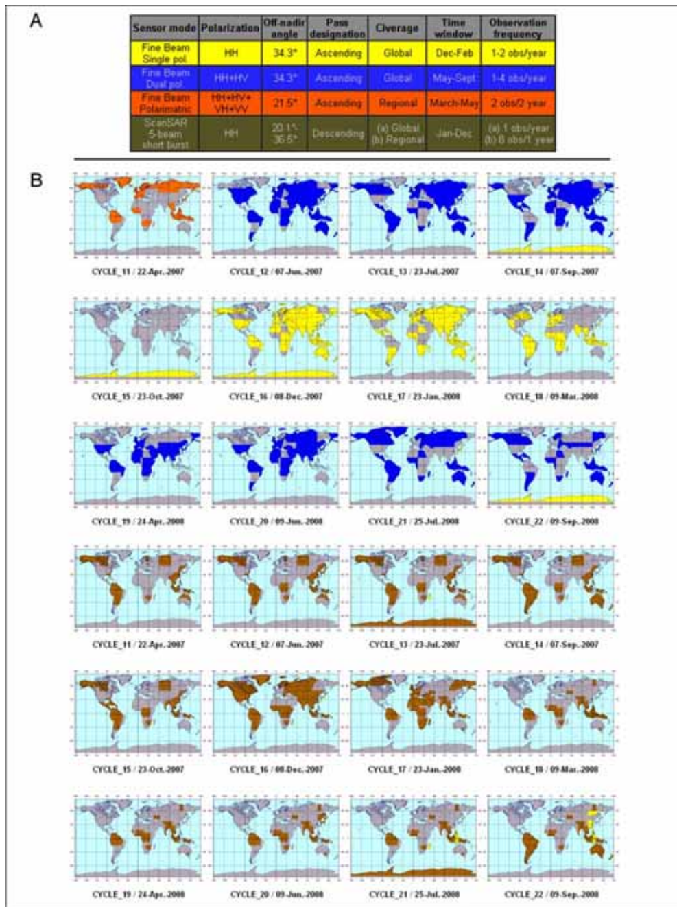
Figure 2.9.1. (A) Global observation strategy for (B) various ALOS/PALSAR sensor modes. The systematic observation strategy is likely to be repeated throughout mission life, projected to last beyond 2016 (source: JAXA/EORC).
