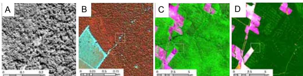
Figure 2.2.2. Unplanned logged forest in Sinop, Mato Grosso, Brazilian Amazon in: (A) Ikonos panchromatic image (1 meter pixel); (B) Ikonos multi-spectral and panchromatic fusion (4 meter pixel); (C) Landsat TM5 multi-spectral (R5, G4, B3; 30 meter pixel); and (D) Normalized Difference Fraction Index (NDFI) image (sub-pixel within 30 m). These images were acquired in August 2001.
