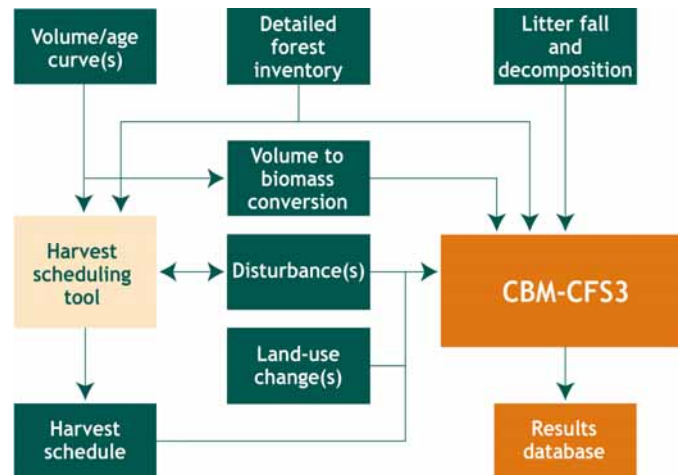
Figure 3.1.2. CBM-CFS3 uses data from forest management planning for national-scale integration of forest C cycle data.
