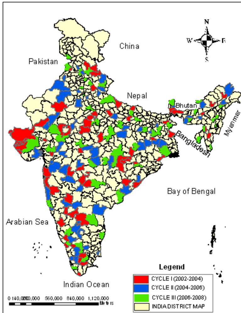
Figure 3.3.1. Selected districts under national forest inventory.
