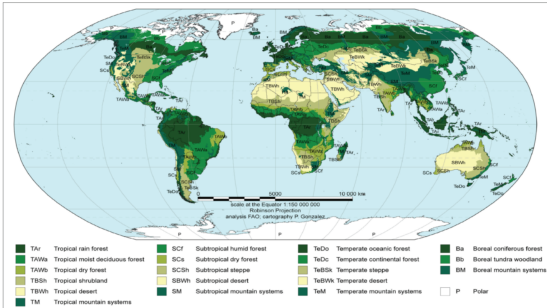
Figure 4.1 Global ecological zones, based on observed climate and vegetation patterns (FAO, 2001). Data for geographic information systems available at http://www.fao.org .
