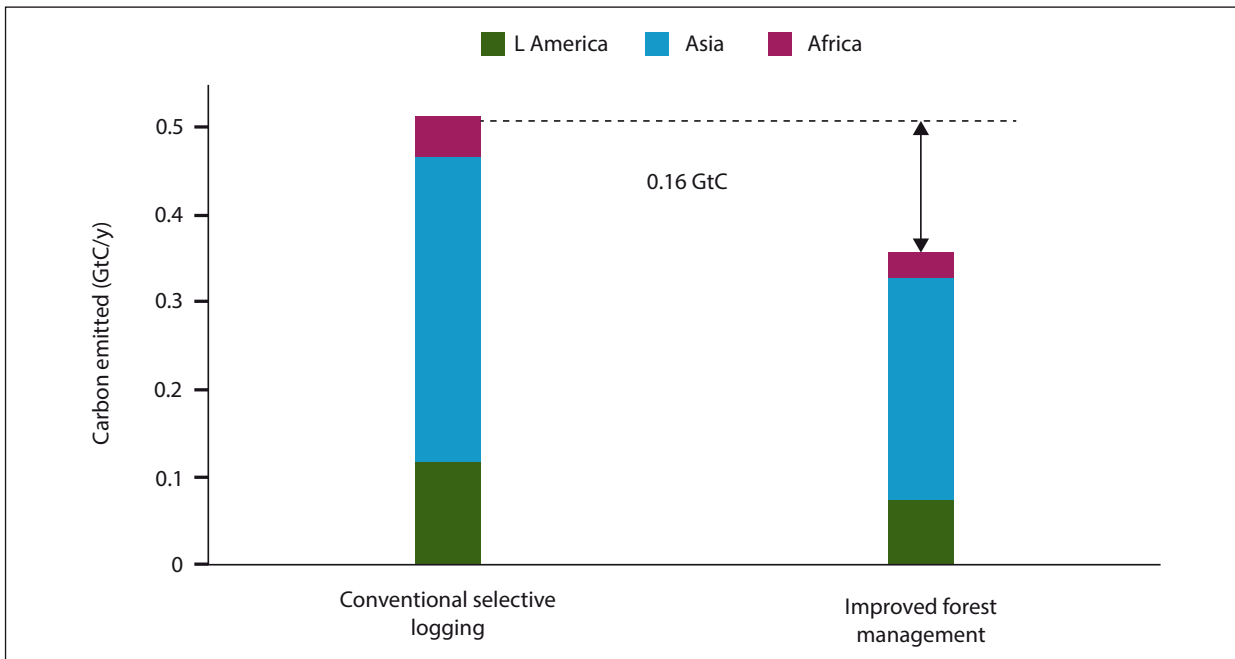
Figure 4.1: Annual Reductions in Global Carbon Emissions that Would Result from Adoption of Improved Tropical Forest Management Practices (Protocol S1)
