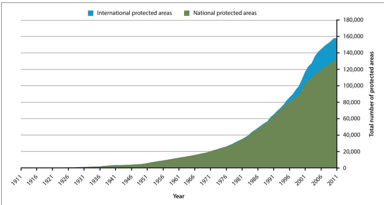
Figure 4.2 – Growth in number of nationally and internationally designated protected areas (1911-2011)
