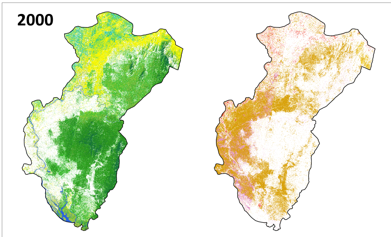
Map 10: Distribution of natural and human-made land cover in 2000 and 2014 (based on NASRDA and FAO 2015 data)
